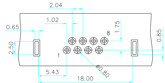
PCB Layout View Component Side Show SCALE 4:1
